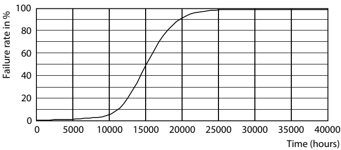
Life Expectancy Diagram - CorePro lustre ND 7-60W E14 865 P48 FR
