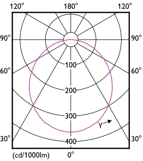
Downlight 59469 MESON 175 40K WH Recessed-LDD
