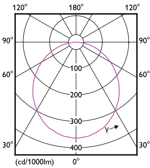
Downlight 59471 MESON 200 40K WH Recessed-LDD
