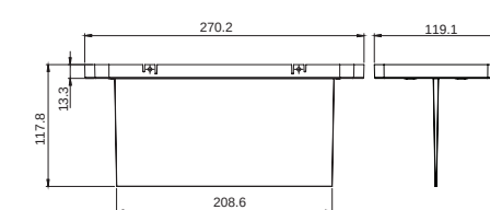
SafeLite 20m Exit Sign Plexiglass drawings (mm)
