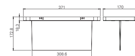
SafeLite 30m Exit Sign Plexiglass drawings (mm)
