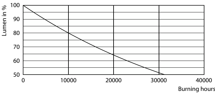
Lumen Maintenance Diagram - CorePro lustre ND 5-40W E14 827 P45 FR
