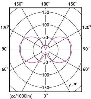
Light Distribution Diagram - CorePro LEDLusterND4.3-40W E14 840P45CLG
