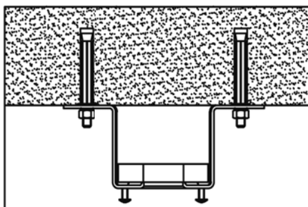
CEILING-MOUNT BRACKET
