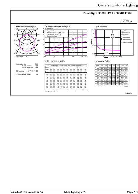
General uniform lighting - DN065B G4 LED20/830 19W 220-240V D200 RD
