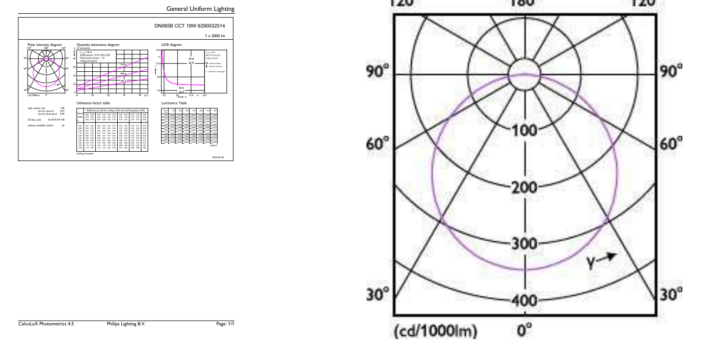
General uniform lighting - DN065B G4 LED20/830_840_865 19W D200 RD
