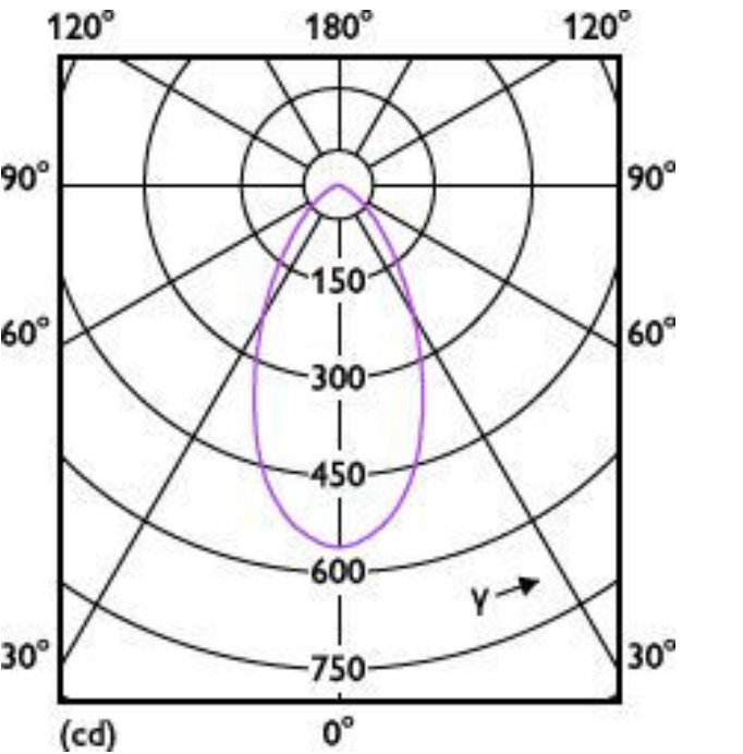
Light Distribution Diagram - RS071B 5S/827_30_40 60D PSR PI6 IP65 WH
